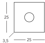
A1337.11.1.VinAu Deckenleuchte / ceiling lamp 1 lp., incl. LED GX53, 7 W 560 lm, 2700 K
