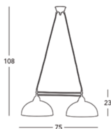
731.82.68 Balken / chandelier 2 l.p., E27, 75W / LED E27
