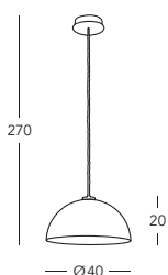
■ A1339.31.Co.VinAu/40 Hängeleuchte / hanging lamp 💡 1 lp., E27, 100W / LED E27
