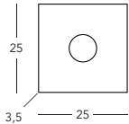
A1337.11.1.Au Deckenleuchte / ceiling lamp 1 lp., incl. LED GX53, 7 W 560 lm, 2700 K
