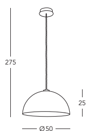
■ A1339.31.Co.VinCu/50 Hängeleuchte / hanging lamp 💡 1 Ip., E27, 100W / LED E27
