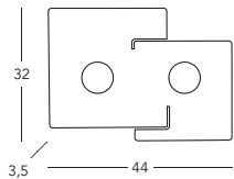
A1337.12.1.Au Deckenleuchte / ceiling lamp 2 lp., incl. LED GX53, 7 W 1120 lm, 2700 K
