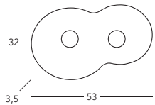
A1336.12.1.SunCu Wandleuchte / wall lamp 2 Ip., incl. LED GX53, 7 W 1120 lm, 2700 K
