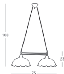
731.82.71 Balken / chandelier 2 l.p., E27, 75W/LED E27
