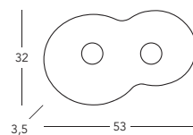
■ A1336.12.1.W Deckenleuchte / ceiling lamp ☐ 2 lp., incl. LED GX53, 7 W 1120 lm, 2700 K
