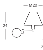
264.61.7 Wandleuchte / wall lamp Messing / brass 1 lp., E14, 40 W / LED E14
