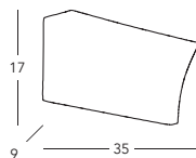
■ 0223.62.W Wandleuchte / wall lamp □ 2 lp., G9, 75 W / LED G9
