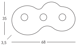
A1336.13.1.Ag Deckenleuchte / ceiling lamp ☑ 3 lp., incl. LED GX53, 7 W 1680 lm, 2700 K
