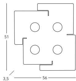
A1337.14.1.Au Deckenleuchte / ceiling lamp 4 lp., incl. LED GX53, 7 W 2240 lm, 2700 K
