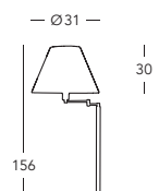
264.41.7 Bodenleuchte / floor lamp Messing / brass 1 lp., E27, 60 W / LED E27
