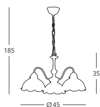
■ 731.83.116 Luster / chandelier 💡 3 lp., E27, 75 W / LED E27
