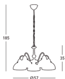
■ 731.85.20 Luster / chandelier □ 5 lp., E27, 75 W / LED E27
