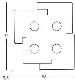
A1337.14.1.VinAu Deckenleuchte / ceiling lamp 4 lp., incl. LED GX53, 7 W 2240 lm, 2700 K
