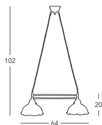
731.82.116 Balken / chandelier 2 Ip., E27, 75 W / LED E27
