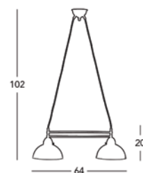
731.82.170 Balken / chandelier 2 l.p., E27, 75W / LED E27
